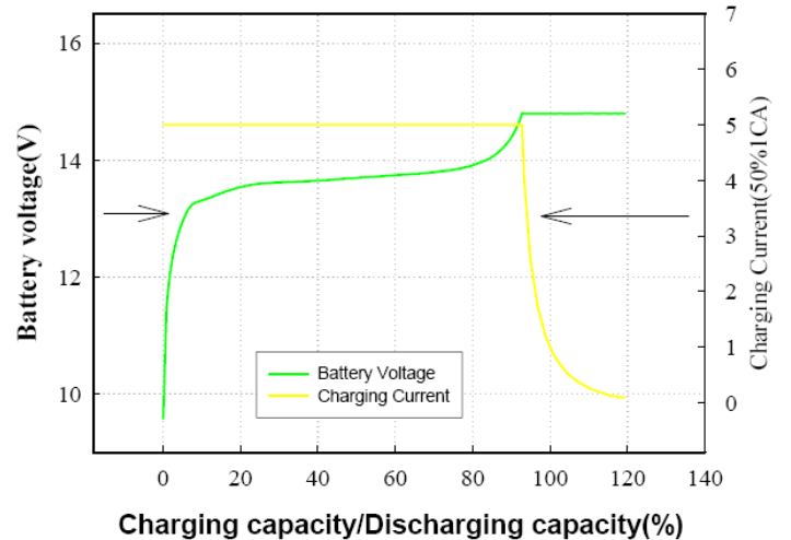
constant voltage charging characteristic (0.5CA, 25Celsius scale)
